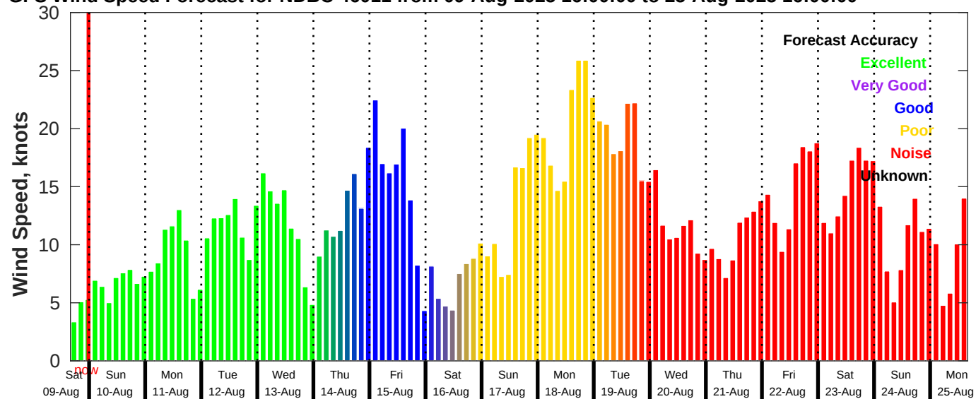
GFS Wind Speed Forecast for NDBC 46011 from 09-Aug-2025 16:00:00 to 25-Aug-2025 16:00:00
