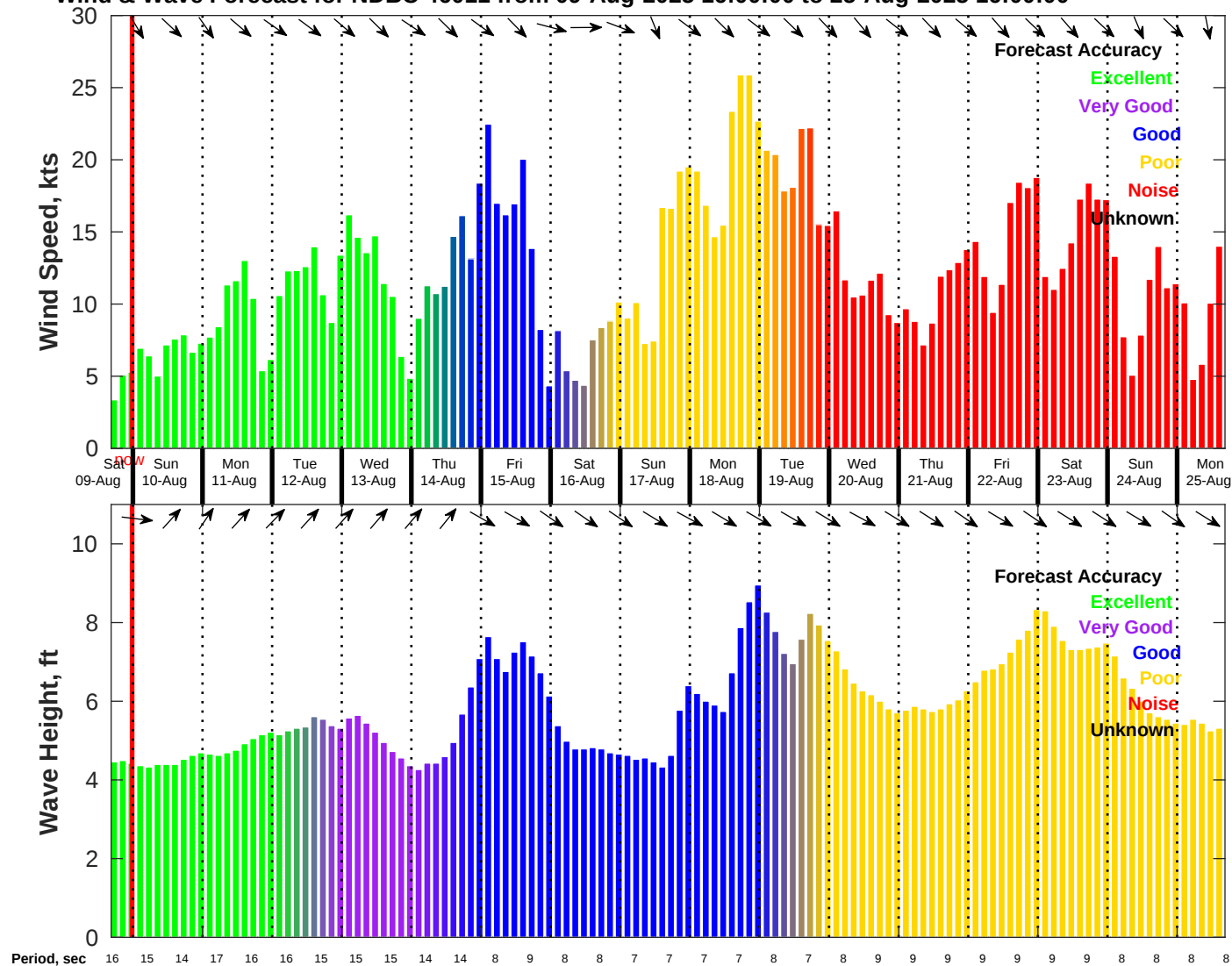
Wind & Wave Forecast for NDBC 46011 from 09-Aug-2025 16:00:00 to 25-Aug-2025 16:00:00
