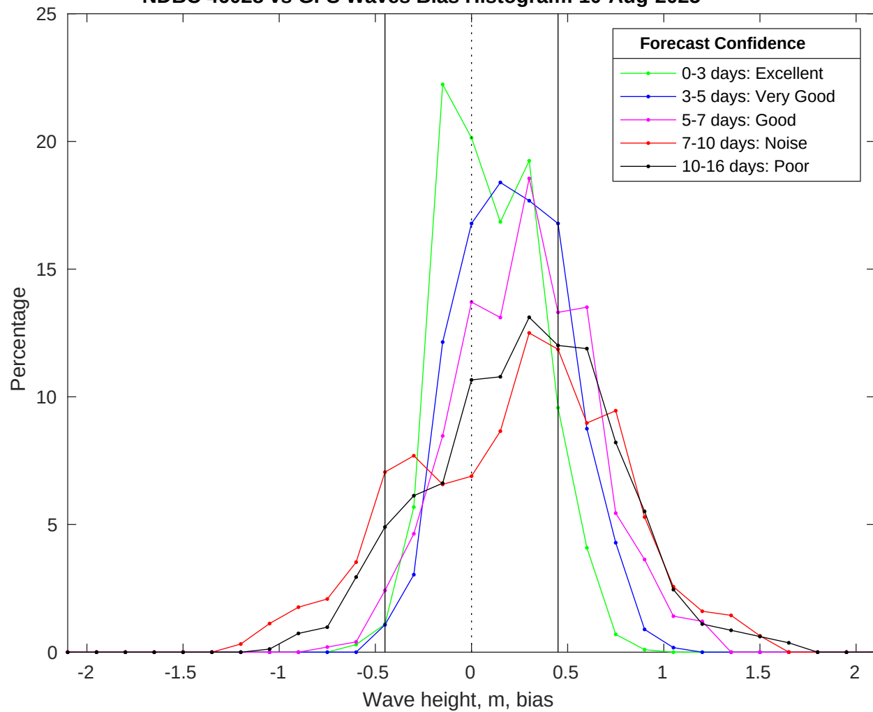
NDBC 46028 vs GFS Waves Bias Histogram: 10-Aug-2025
