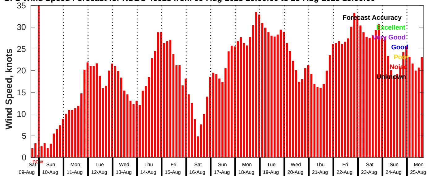
GFS Wind Speed Forecast for NDBC 46028 from 09-Aug-2025 16:00:00 to 25-Aug-2025 16:00:00
