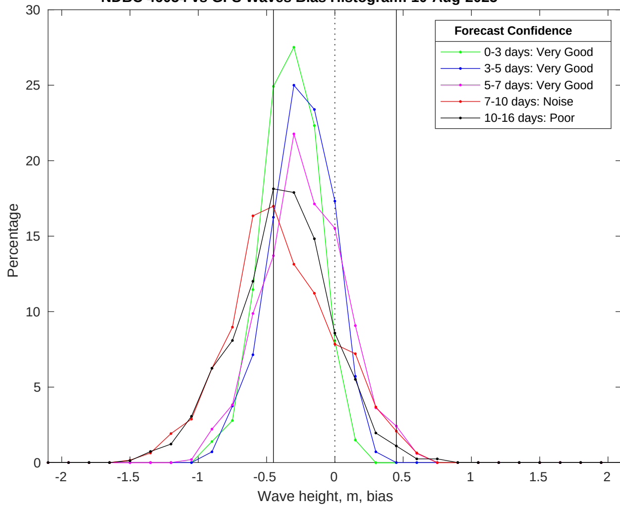
NDBC 46054 vs GFS Waves Bias Histogram: 10-Aug-2025
