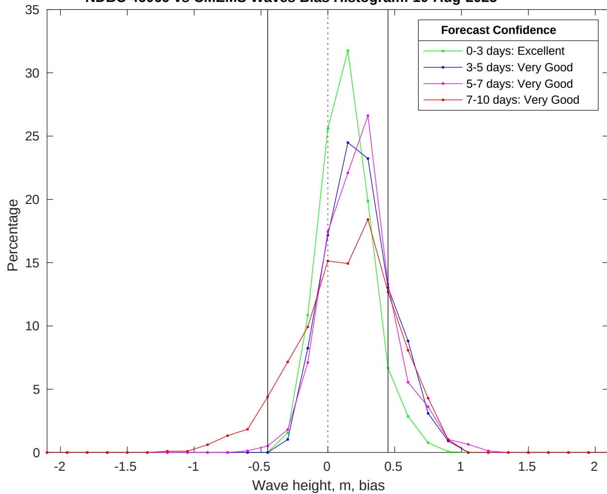
NDBC 46069 vs CMEMS Waves Bias Histogram: 10-Aug-2025
