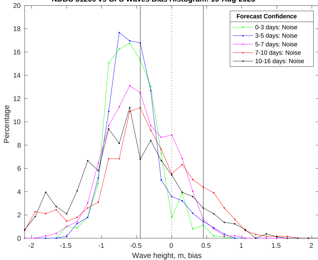
NDBC 51209 vs GFS Waves Bias Histogram: 10-Aug-2025
