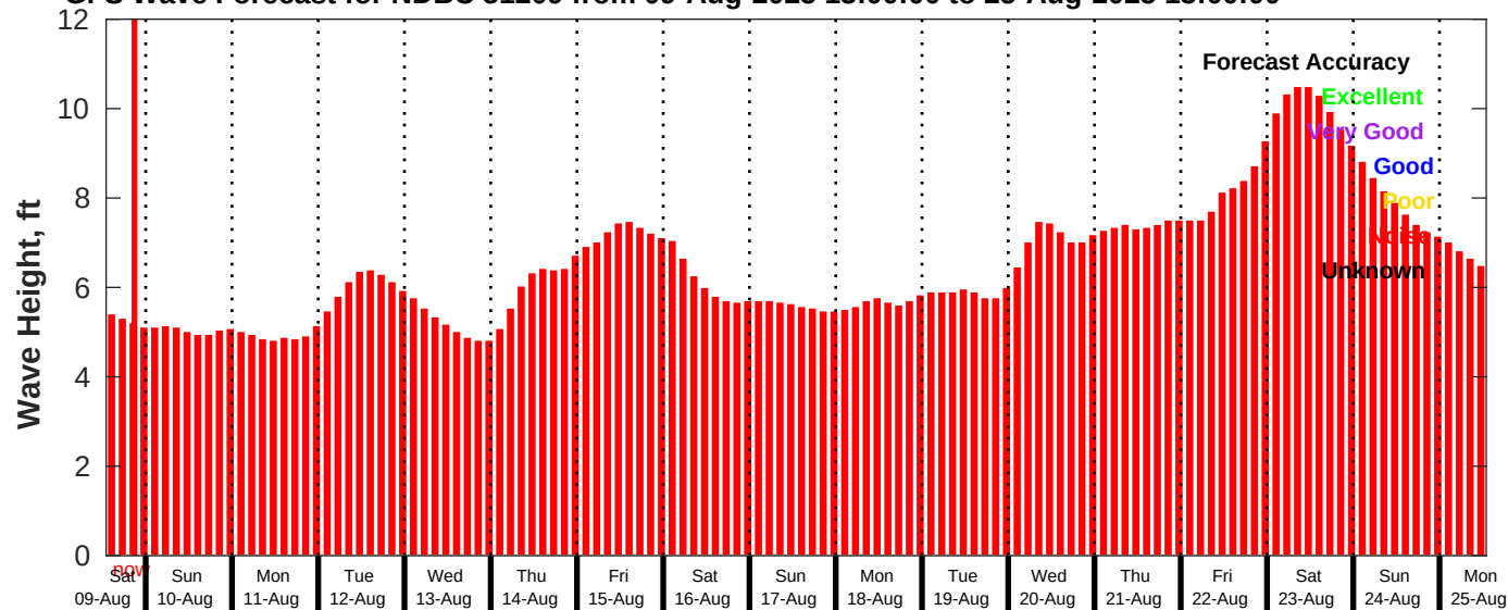
GFS Wave Forecast for NDBC 51209 from 09-Aug-2025 13:00:00 to 25-Aug-2025 13:00:00
