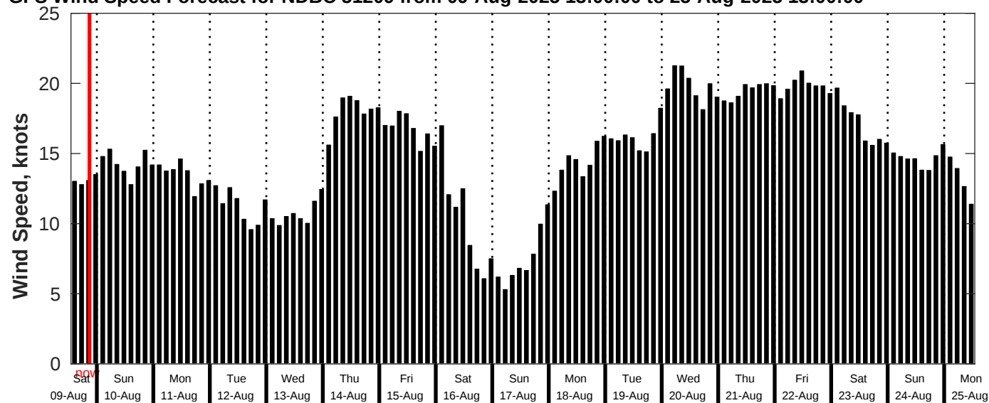
GFS Wind Speed Forecast for NDBC 51209 from 09-Aug-2025 13:00:00 to 25-Aug-2025 13:00:00
