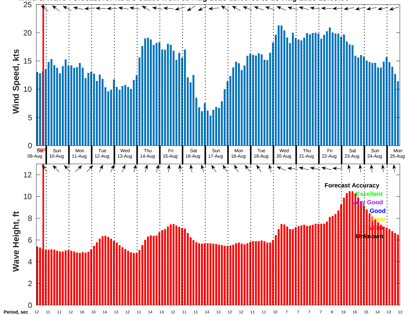
Wind & Wave Forecast for NDBC 51209 from 09-Aug-2025 13:00:00 to 25-Aug-2025 13:00:00
