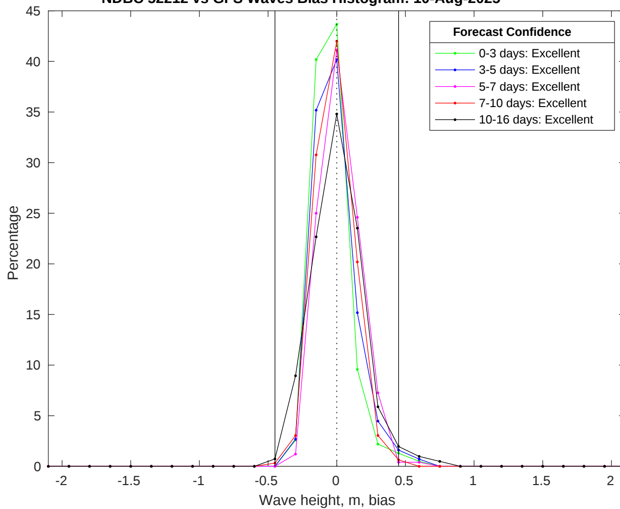
NDBC 52212 vs GFS Waves Bias Histogram: 10-Aug-2025
