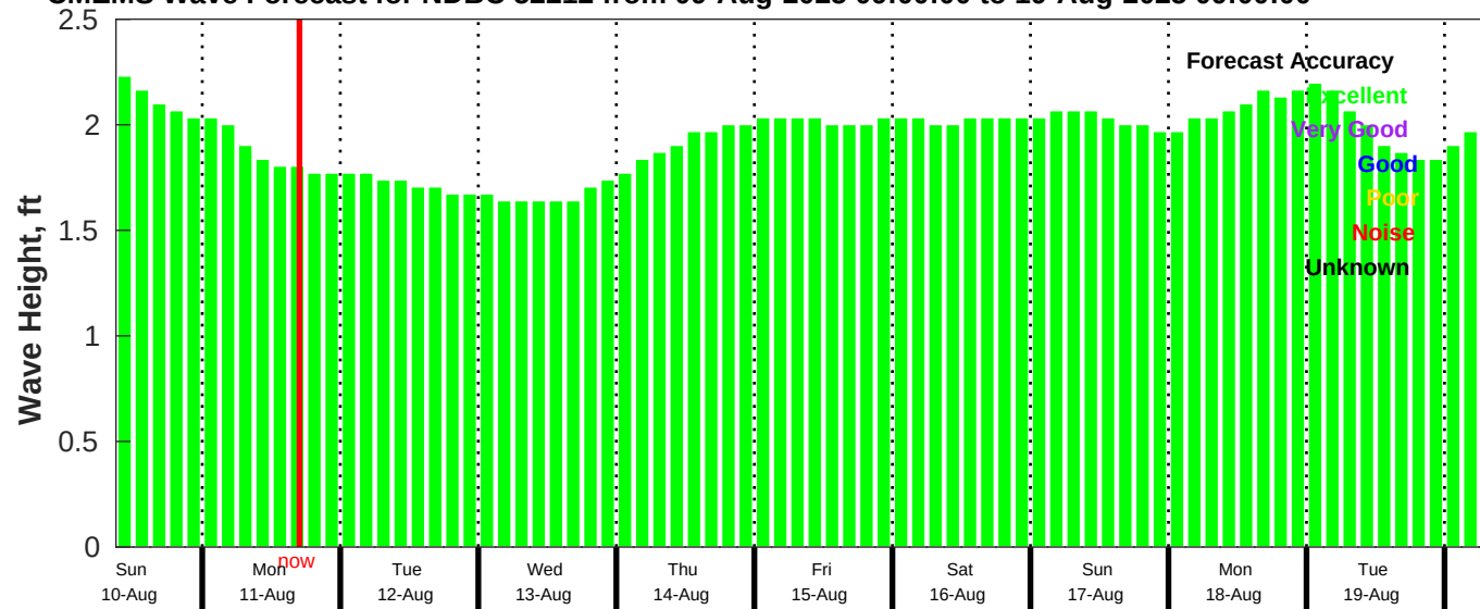
CMEMS Wave Forecast for NDBC 52212 from 09-Aug-2025 09:00:00 to 19-Aug-2025 09:00:00
