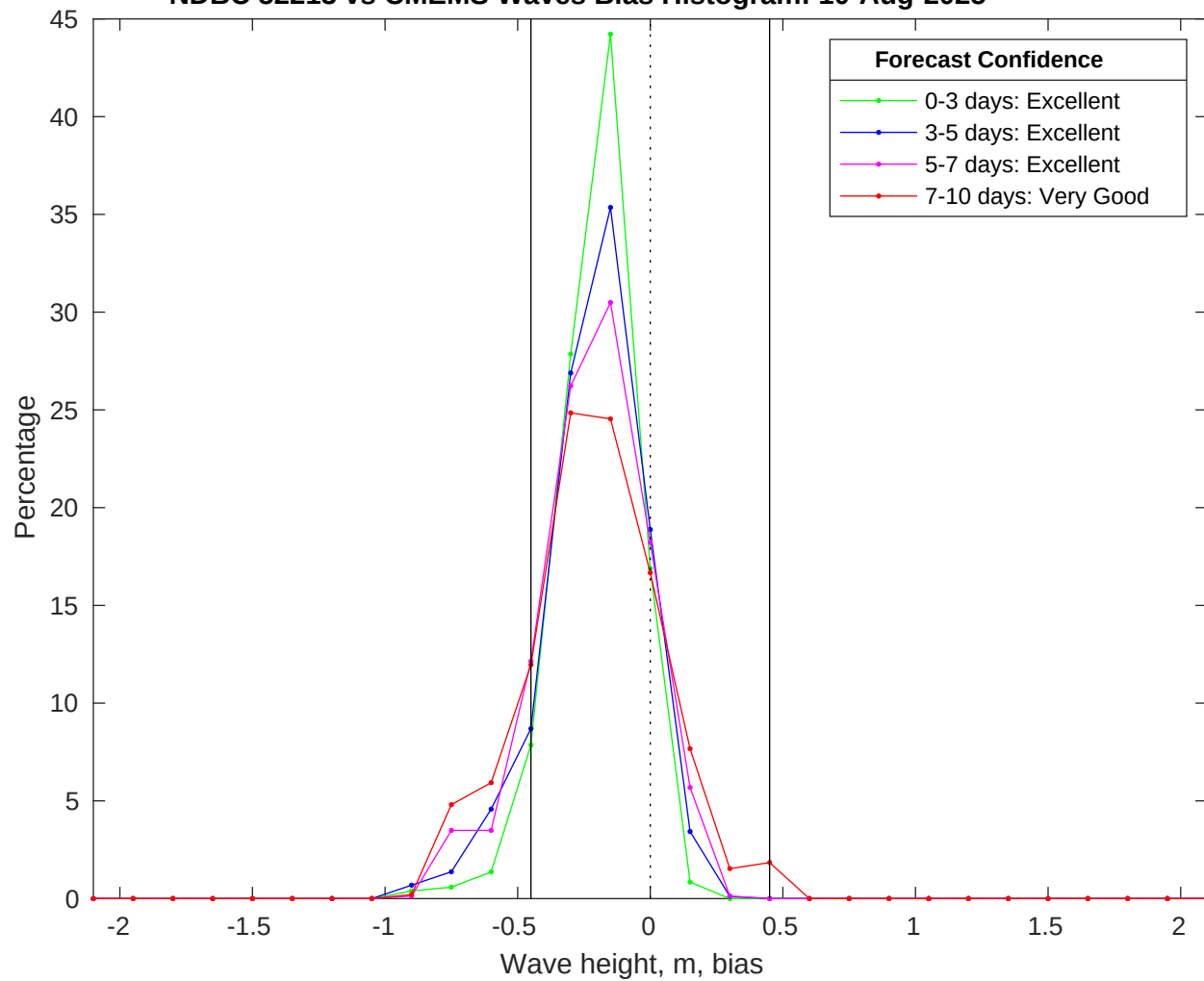
NDBC 52213 vs CMEMS Waves Bias Histogram: 10-Aug-2025
