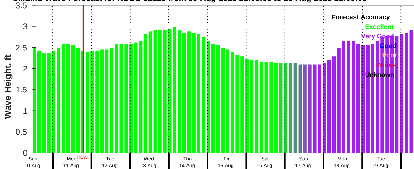
CMEMS Wave Forecast for NDBC 52213 from 09-Aug-2025 11:00:00 to 19-Aug-2025 11:00:00
