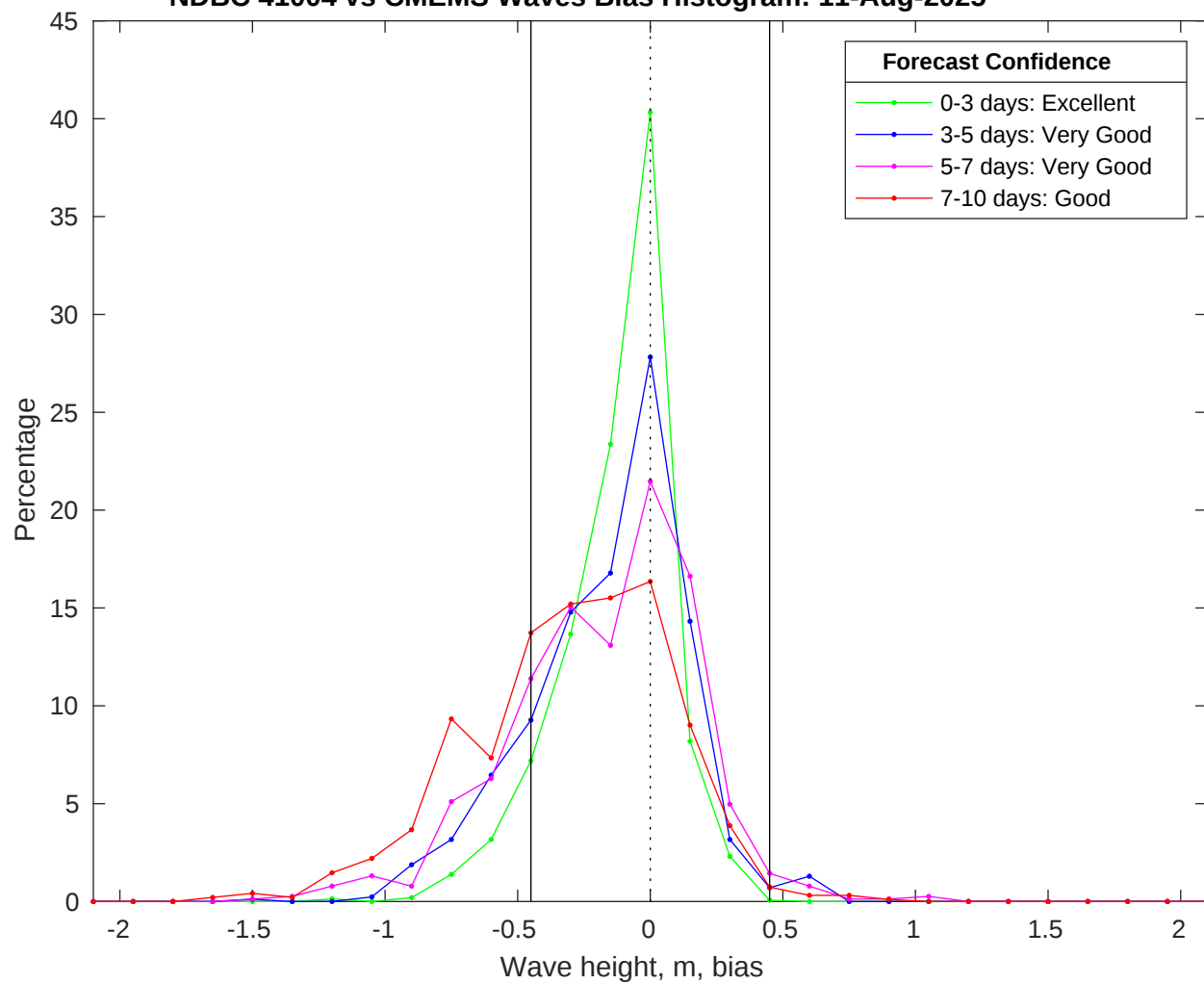
NDBC 41004 vs CMEMS Waves Bias Histogram: 11-Aug-2025
