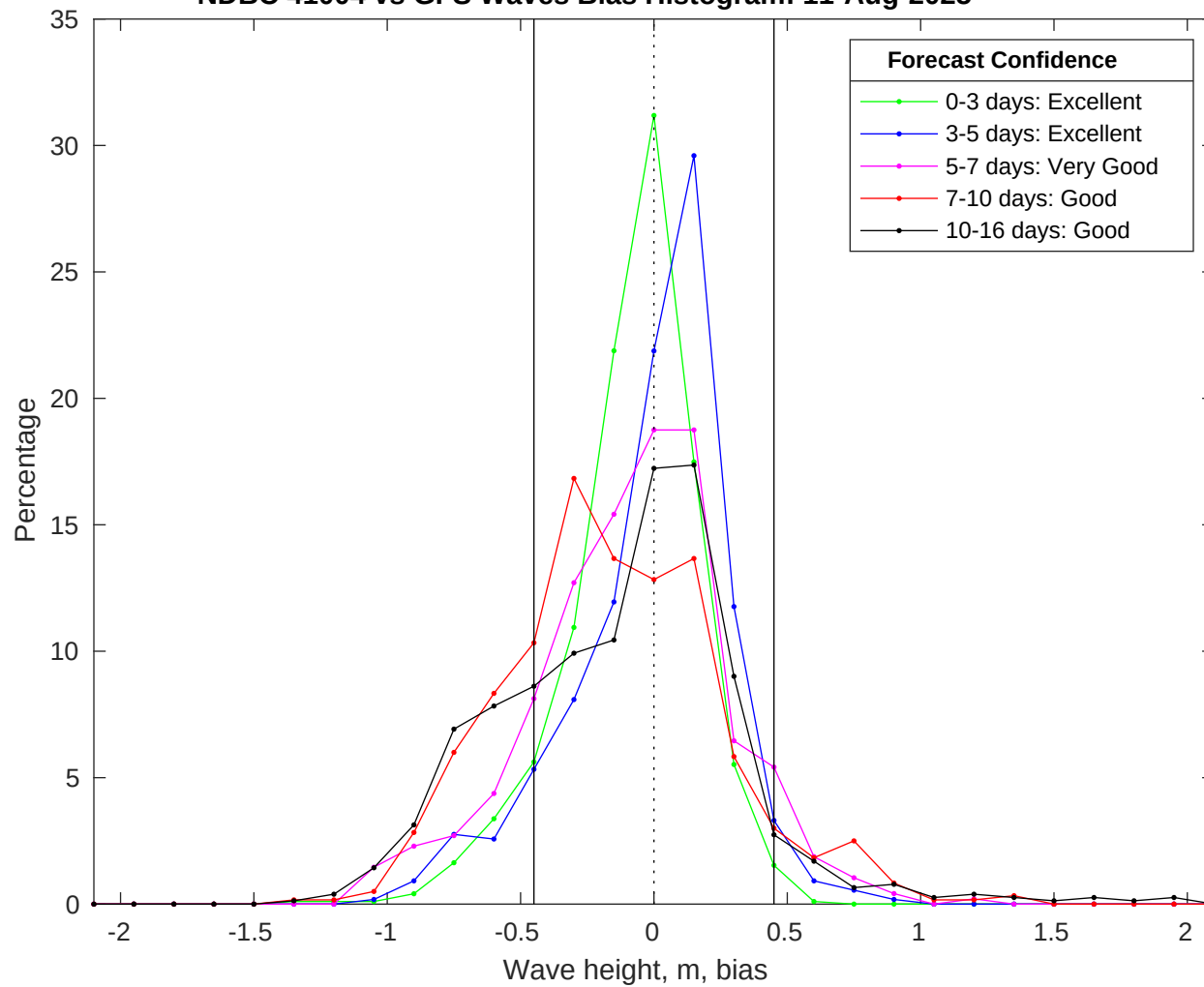
NDBC 41004 vs GFS Waves Bias Histogram: 11-Aug-2025
