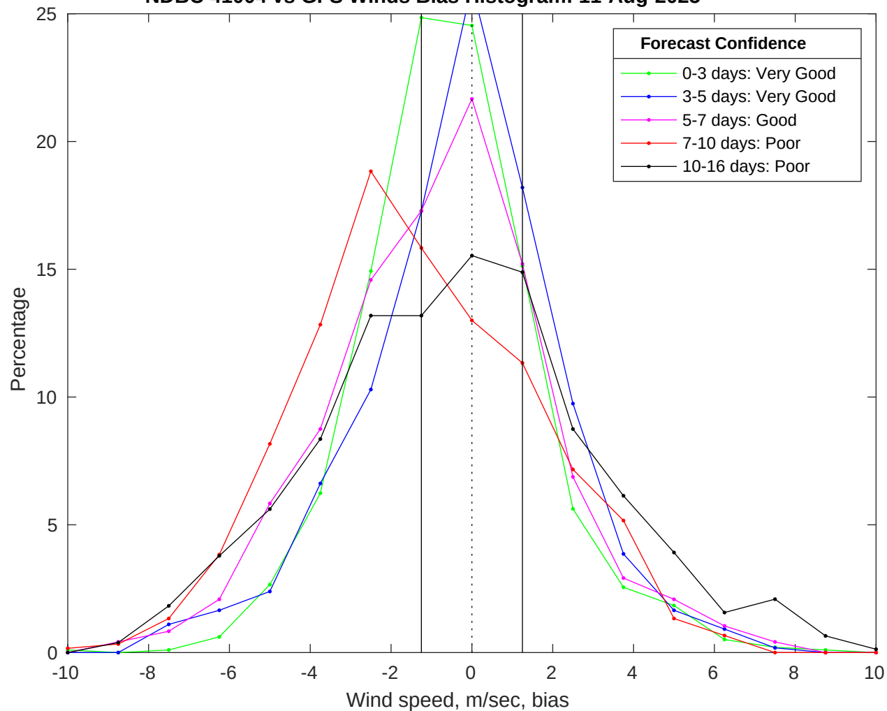
NDBC 41004 vs GFS Winds Bias Histogram: 11-Aug-2025
