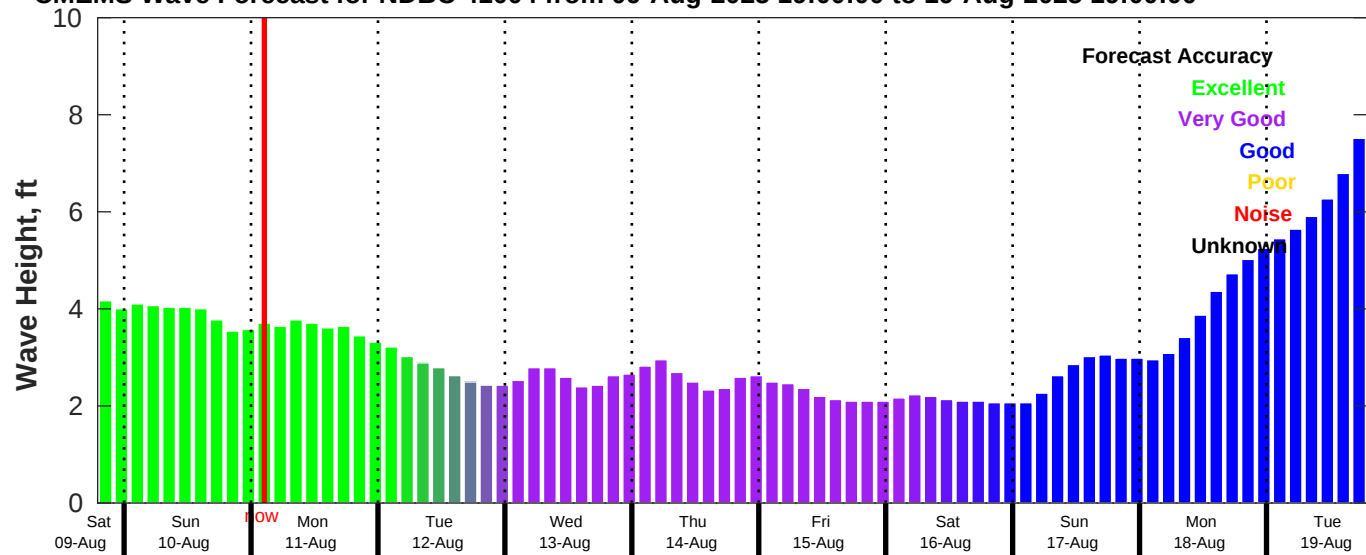
CMEMS Wave Forecast for NDBC 41004 from 09-Aug-2025 19:00:00 to 19-Aug-2025 19:00:00
