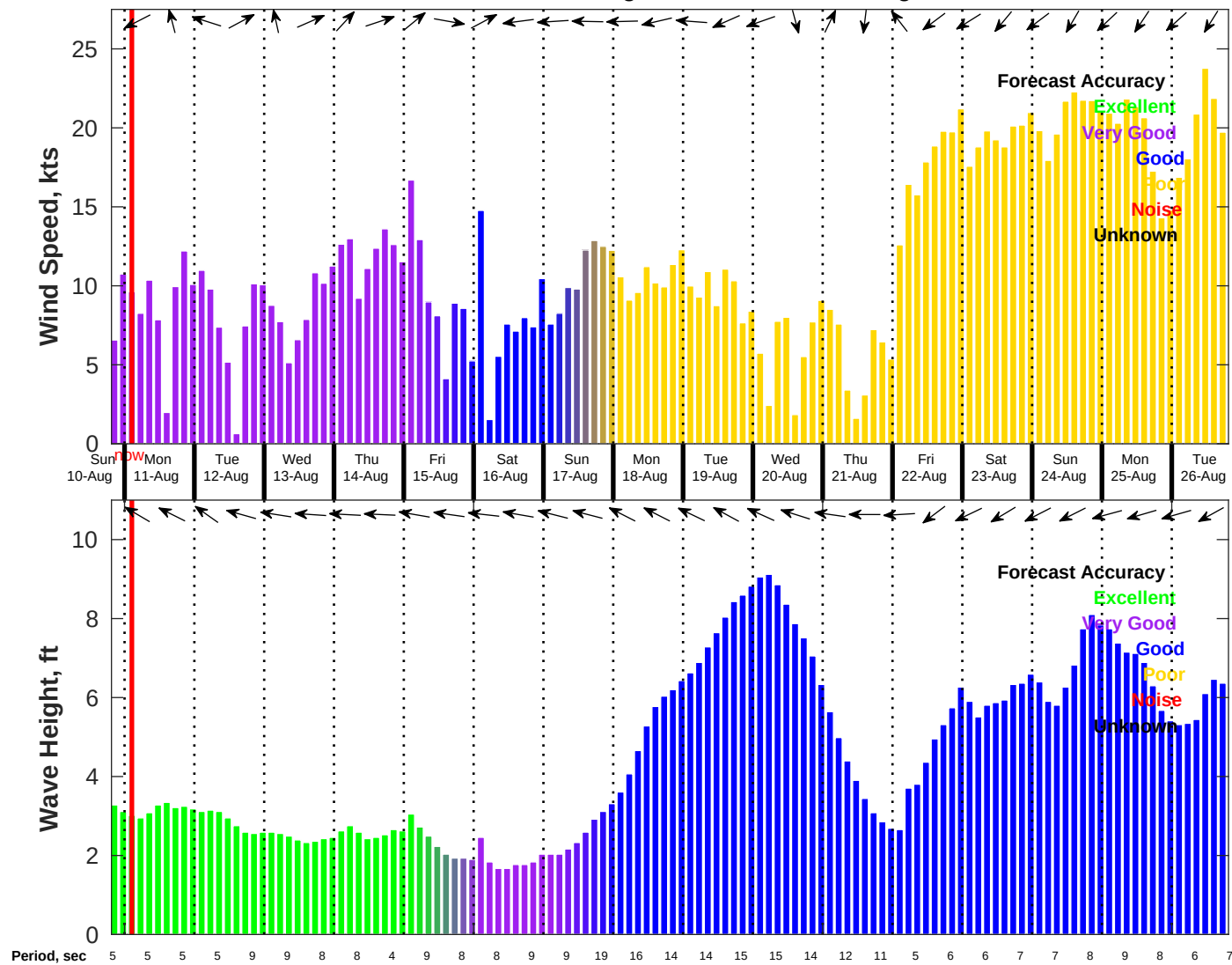
Wind & Wave Forecast for NDBC 41004 from 10-Aug-2025 19:00:00 to 26-Aug-2025 19:00:00
