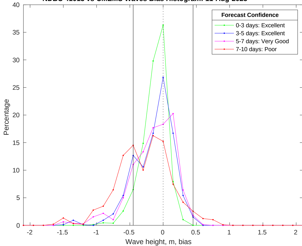
NDBC 41013 vs CMEMS Waves Bias Histogram: 11-Aug-2025
