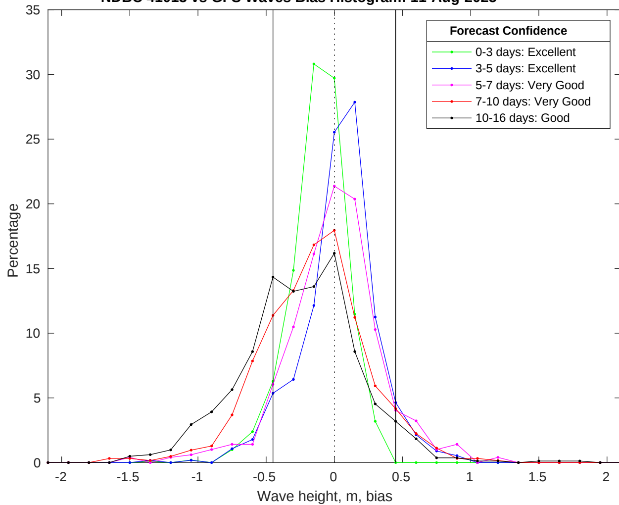
NDBC 41013 vs GFS Waves Bias Histogram: 11-Aug-2025
