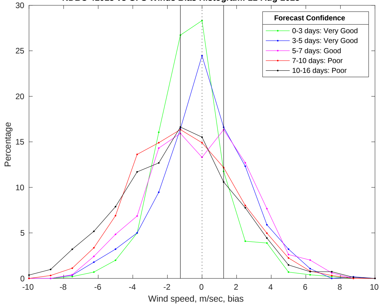
NDBC 41013 vs GFS Winds Bias Histogram: 11-Aug-2025
