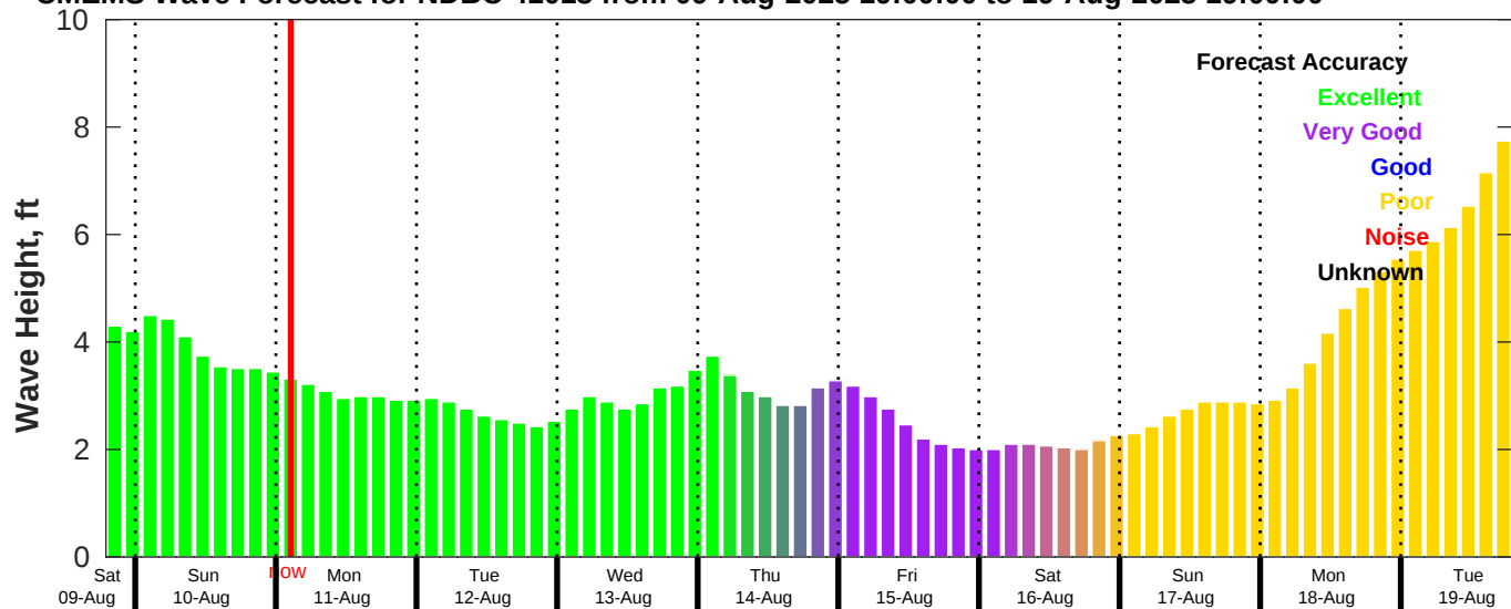
CMEMS Wave Forecast for NDBC 41013 from 09-Aug-2025 19:00:00 to 19-Aug-2025 19:00:00
