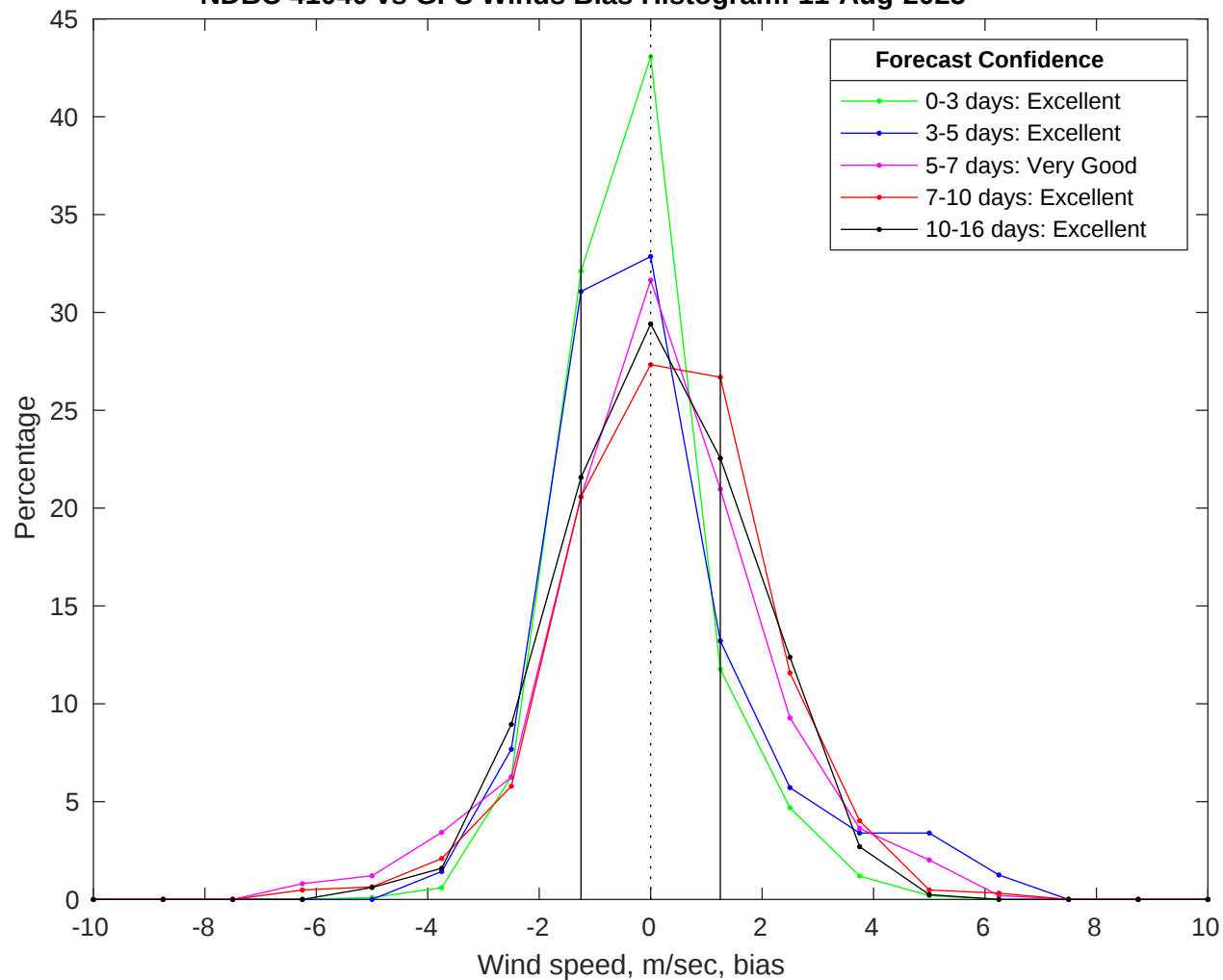
NDBC 41040 vs GFS Winds Bias Histogram: 11-Aug-2025
