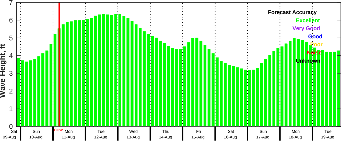
CMEMS Wave Forecast for NDBC 41040 from 09-Aug-2025 21:00:00 to 19-Aug-2025 21:00:00
