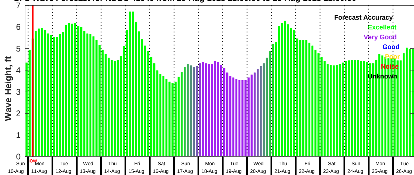
GFS Wave Forecast for NDBC 41040 from 10-Aug-2025 21:00:00 to 26-Aug-2025 21:00:00
