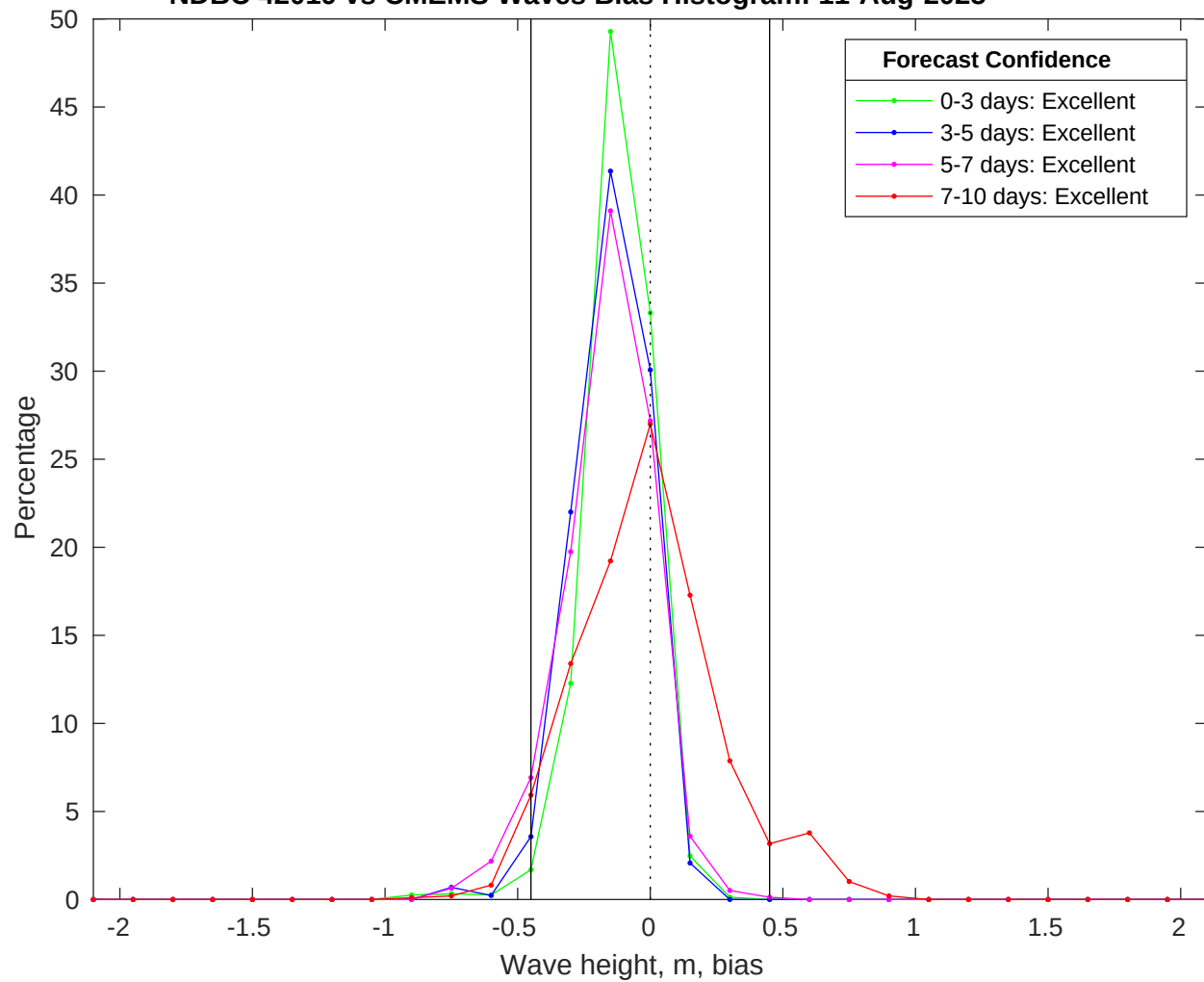
NDBC 42019 vs CMEMS Waves Bias Histogram: 11-Aug-2025
