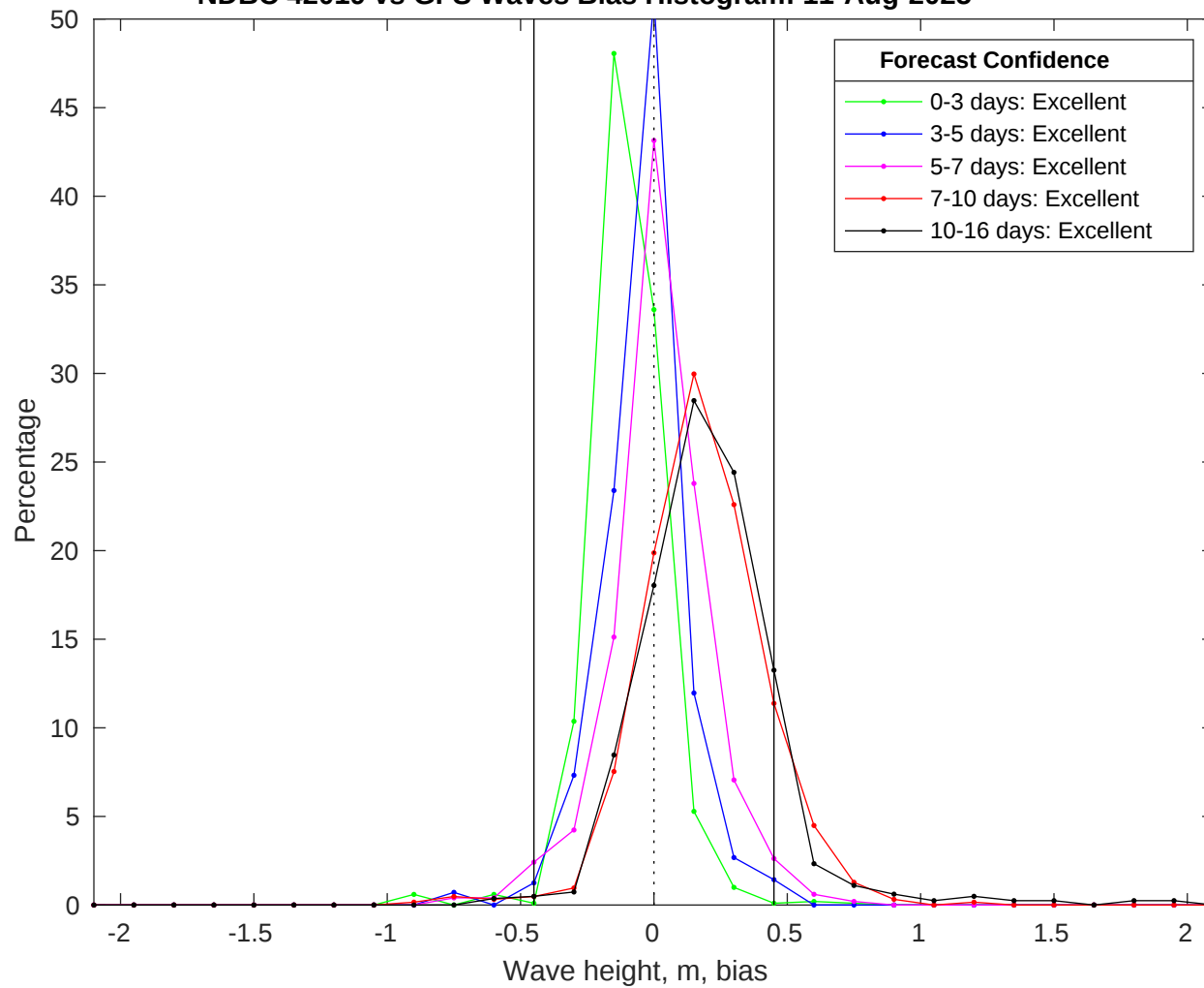
NDBC 42019 vs GFS Waves Bias Histogram: 11-Aug-2025
