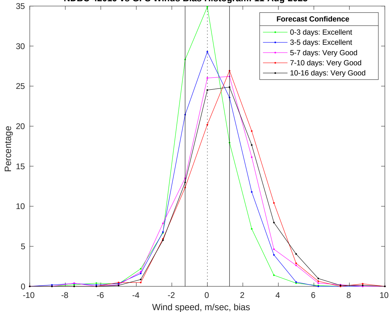
NDBC 42019 vs GFS Winds Bias Histogram: 11-Aug-2025
