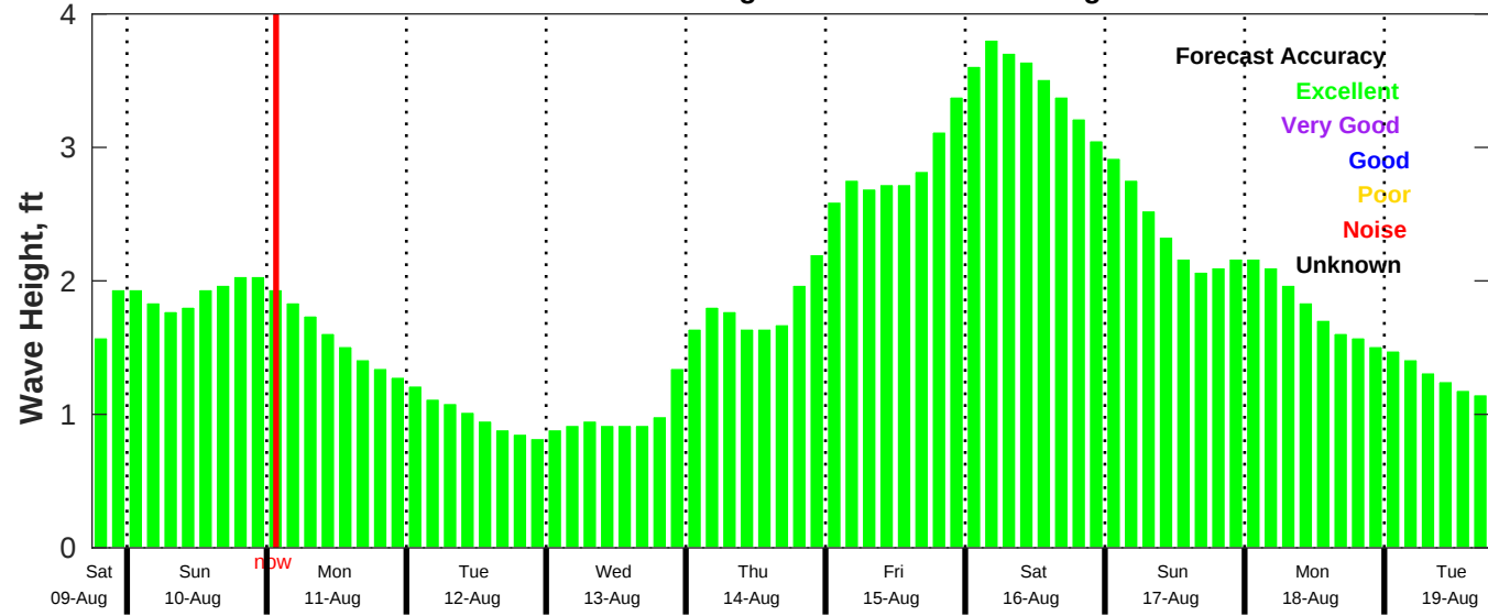
CMEMS Wave Forecast for NDBC 42019 from 09-Aug-2025 18:00:00 to 19-Aug-2025 18:00:00
