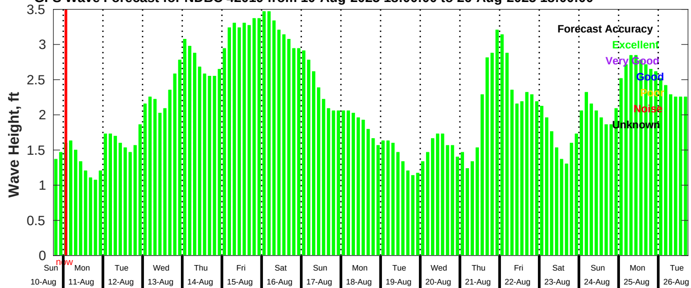
GFS Wave Forecast for NDBC 42019 from 10-Aug-2025 18:00:00 to 26-Aug-2025 18:00:00
