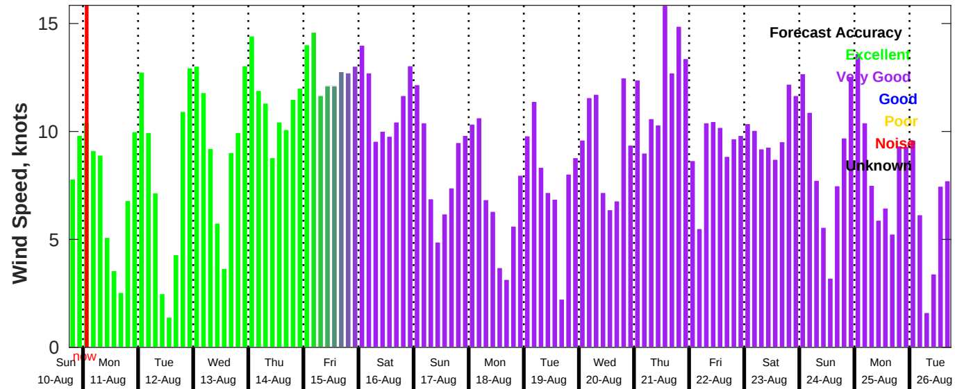
GFS Wind Speed Forecast for NDBC 42019 from 10-Aug-2025 18:00:00 to 26-Aug-2025 18:00:00
