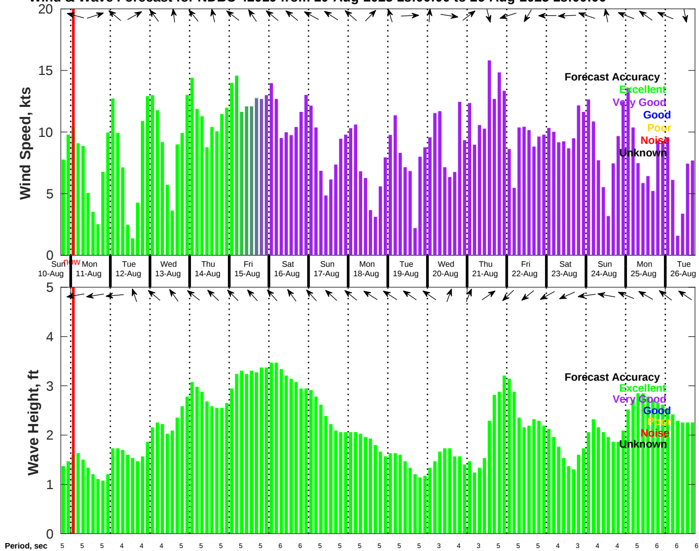
Wind & Wave Forecast for NDBC 42019 from 10-Aug-2025 18:00:00 to 26-Aug-2025 18:00:00
