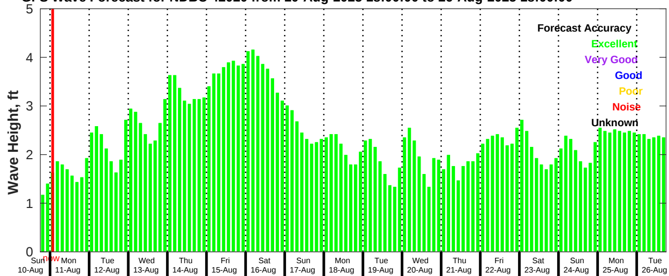
GFS Wave Forecast for NDBC 42020 from 10-Aug-2025 18:00:00 to 26-Aug-2025 18:00:00
