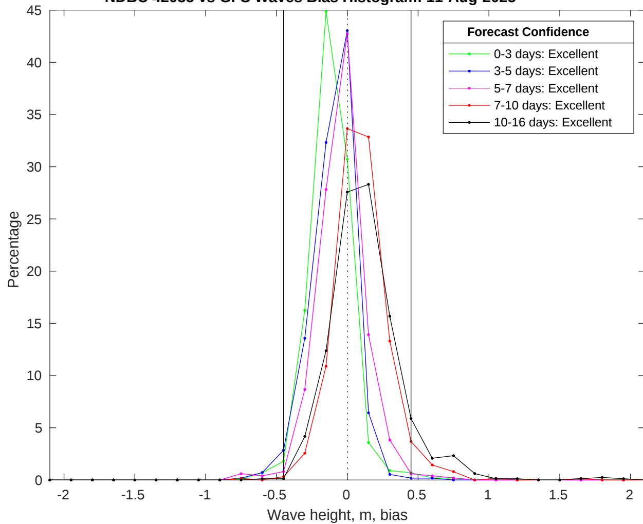
NDBC 42035 vs GFS Waves Bias Histogram: 11-Aug-2025
