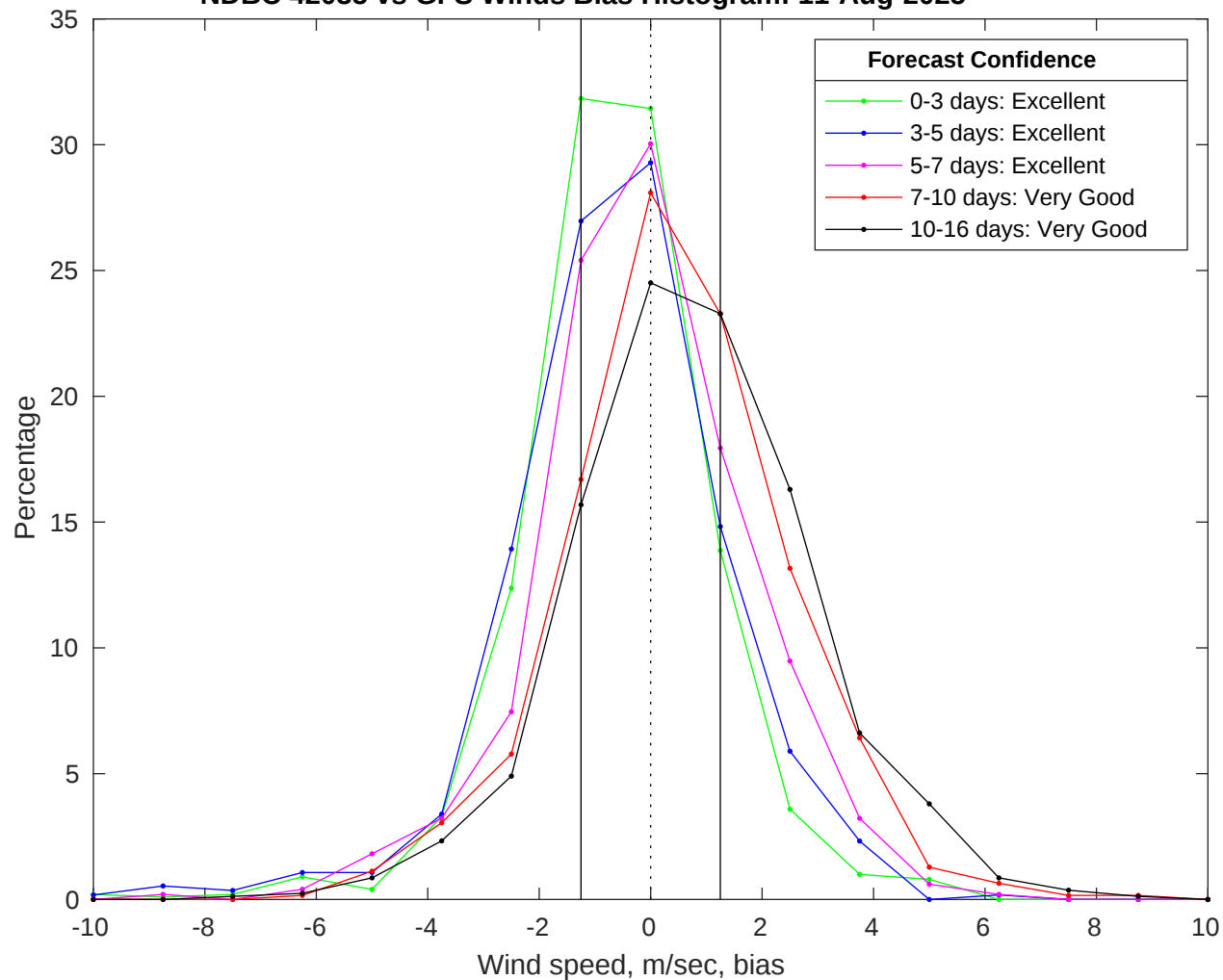
NDBC 42035 vs GFS Winds Bias Histogram: 11-Aug-2025
