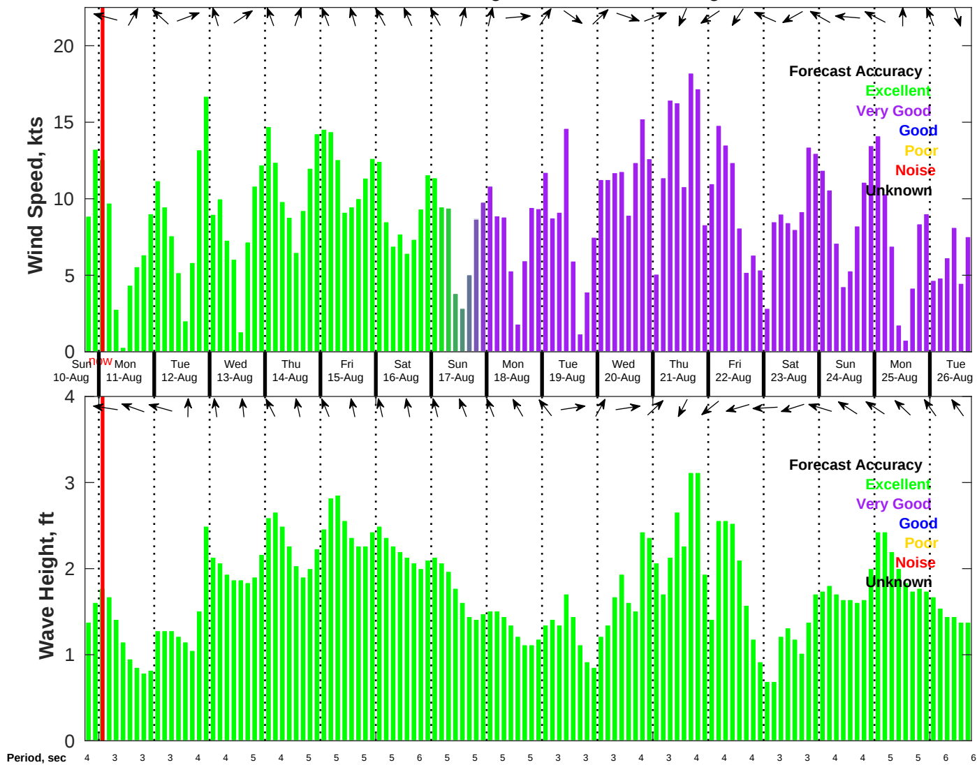
Wind & Wave Forecast for NDBC 42035 from 10-Aug-2025 18:00:00 to 26-Aug-2025 18:00:00
