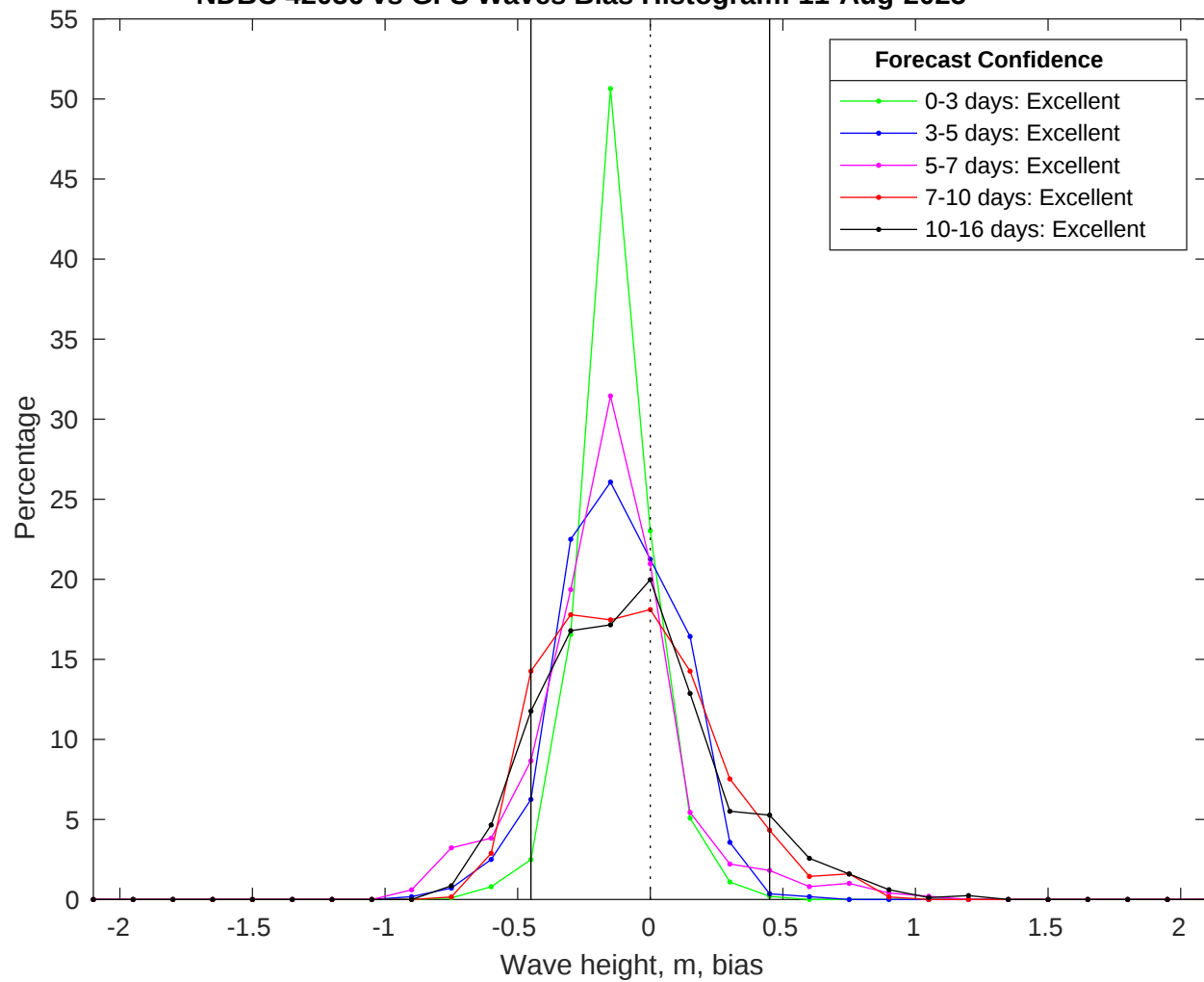
NDBC 42036 vs GFS Waves Bias Histogram: 11-Aug-2025
