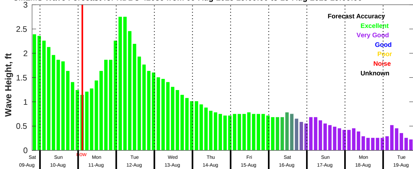
CMEMS Wave Forecast for NDBC 42036 from 09-Aug-2025 19:00:00 to 19-Aug-2025 19:00:00
