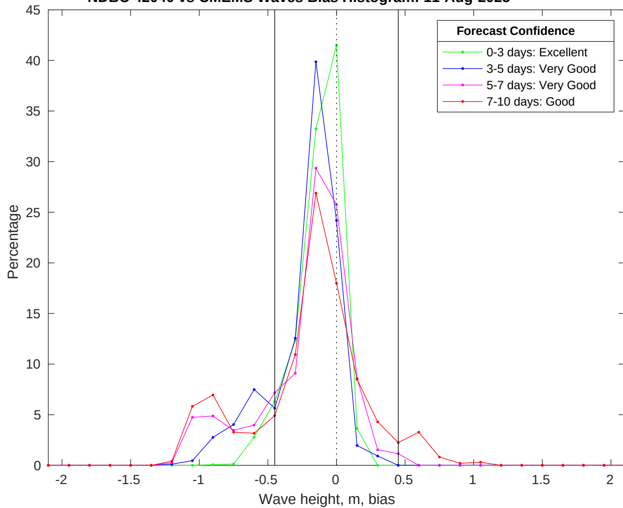
NDBC 42040 vs CMEMS Waves Bias Histogram: 11-Aug-2025
