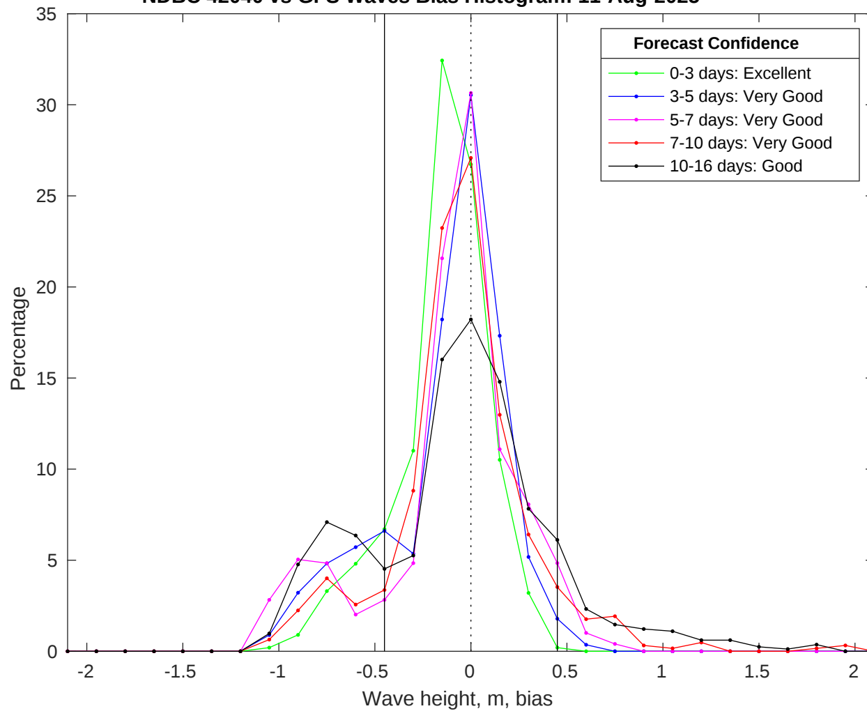
NDBC 42040 vs GFS Waves Bias Histogram: 11-Aug-2025
