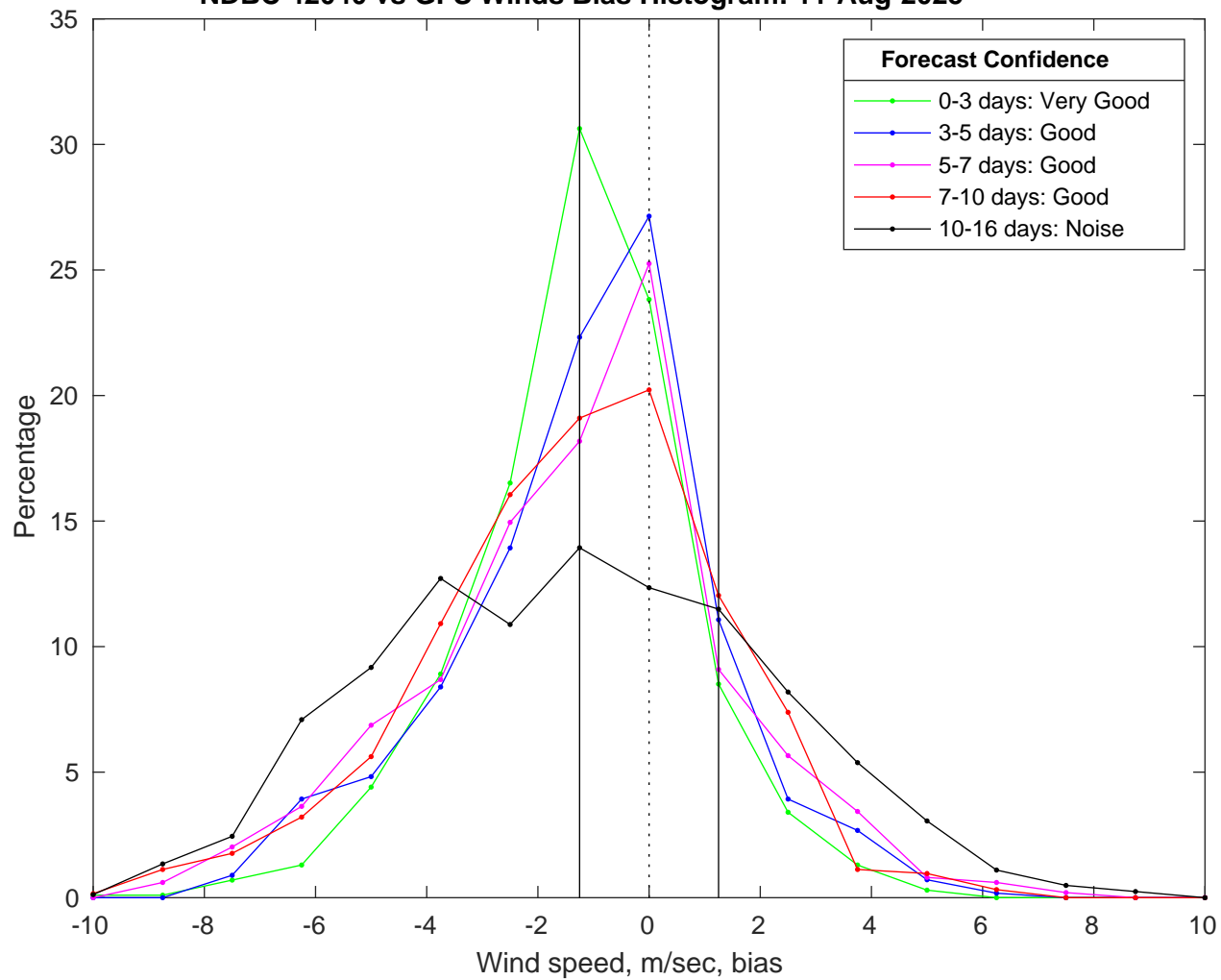
NDBC 42040 vs GFS Winds Bias Histogram: 11-Aug-2025
