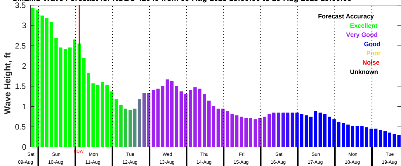
CMEMS Wave Forecast for NDBC 42040 from 09-Aug-2025 19:00:00 to 19-Aug-2025 19:00:00
