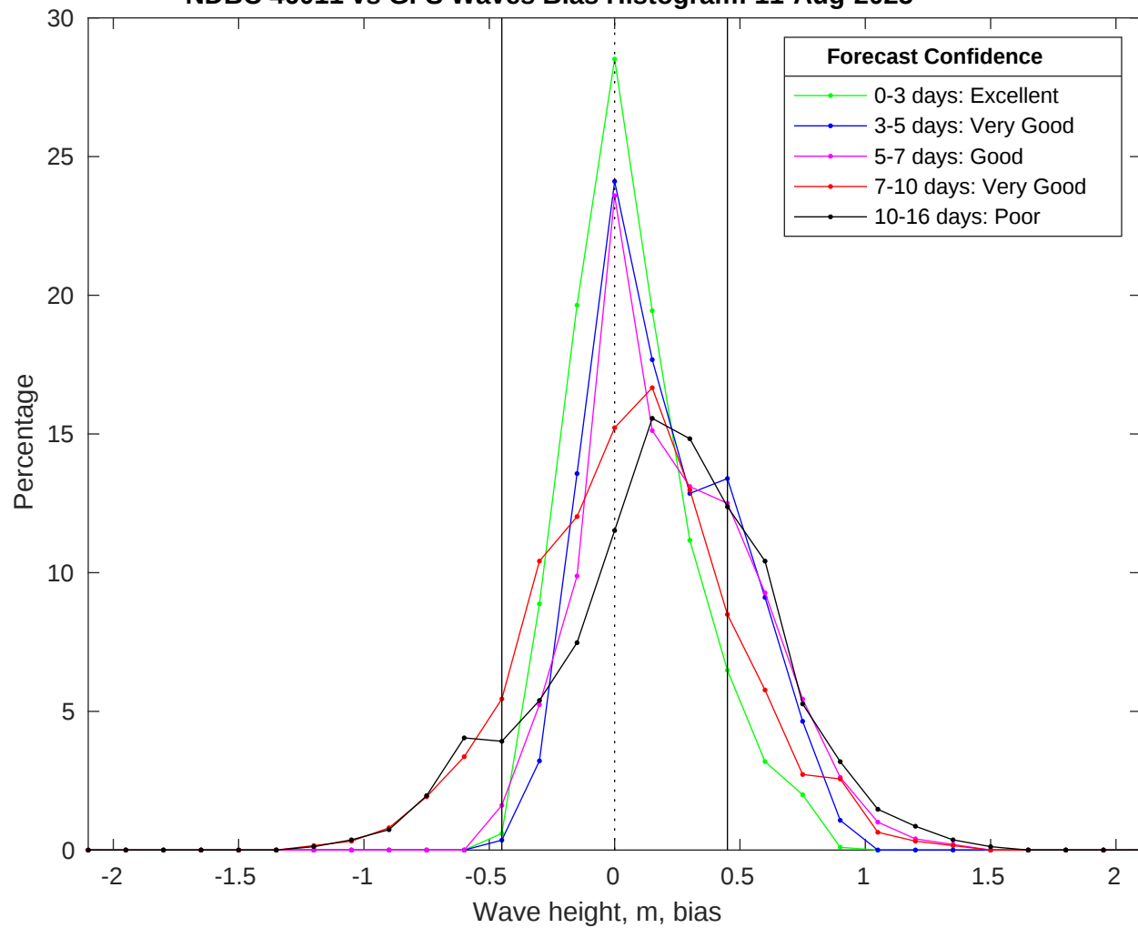
NDBC 46011 vs GFS Waves Bias Histogram: 11-Aug-2025
