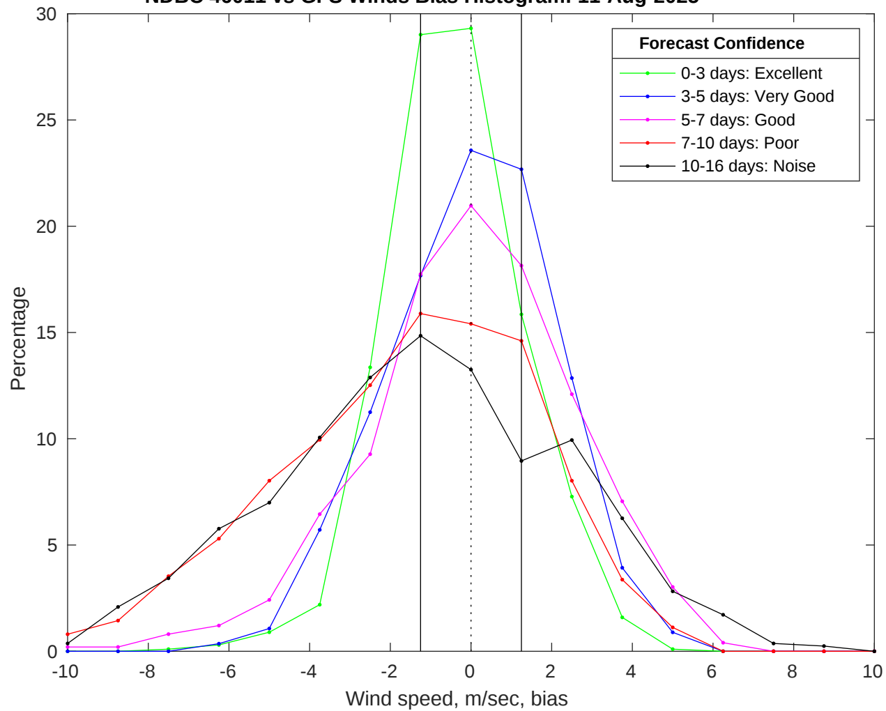
NDBC 46011 vs GFS Winds Bias Histogram: 11-Aug-2025
