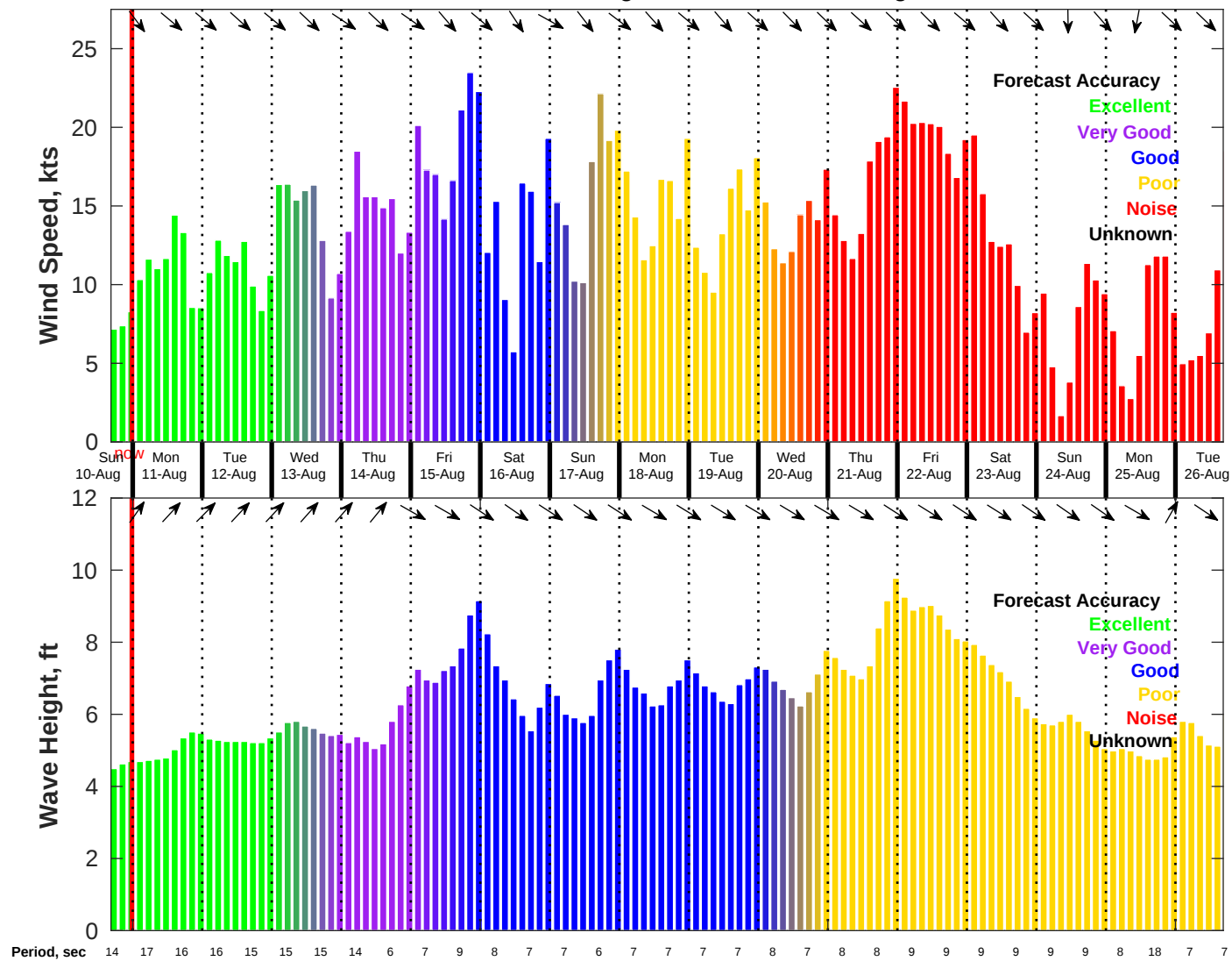
Wind & Wave Forecast for NDBC 46011 from 10-Aug-2025 16:00:00 to 26-Aug-2025 16:00:00
