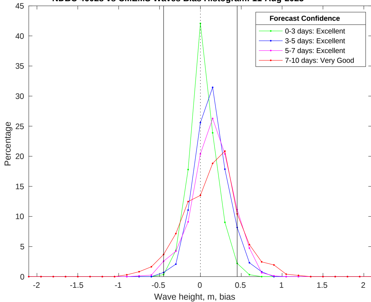
NDBC 46028 vs CMEMS Waves Bias Histogram: 11-Aug-2025
