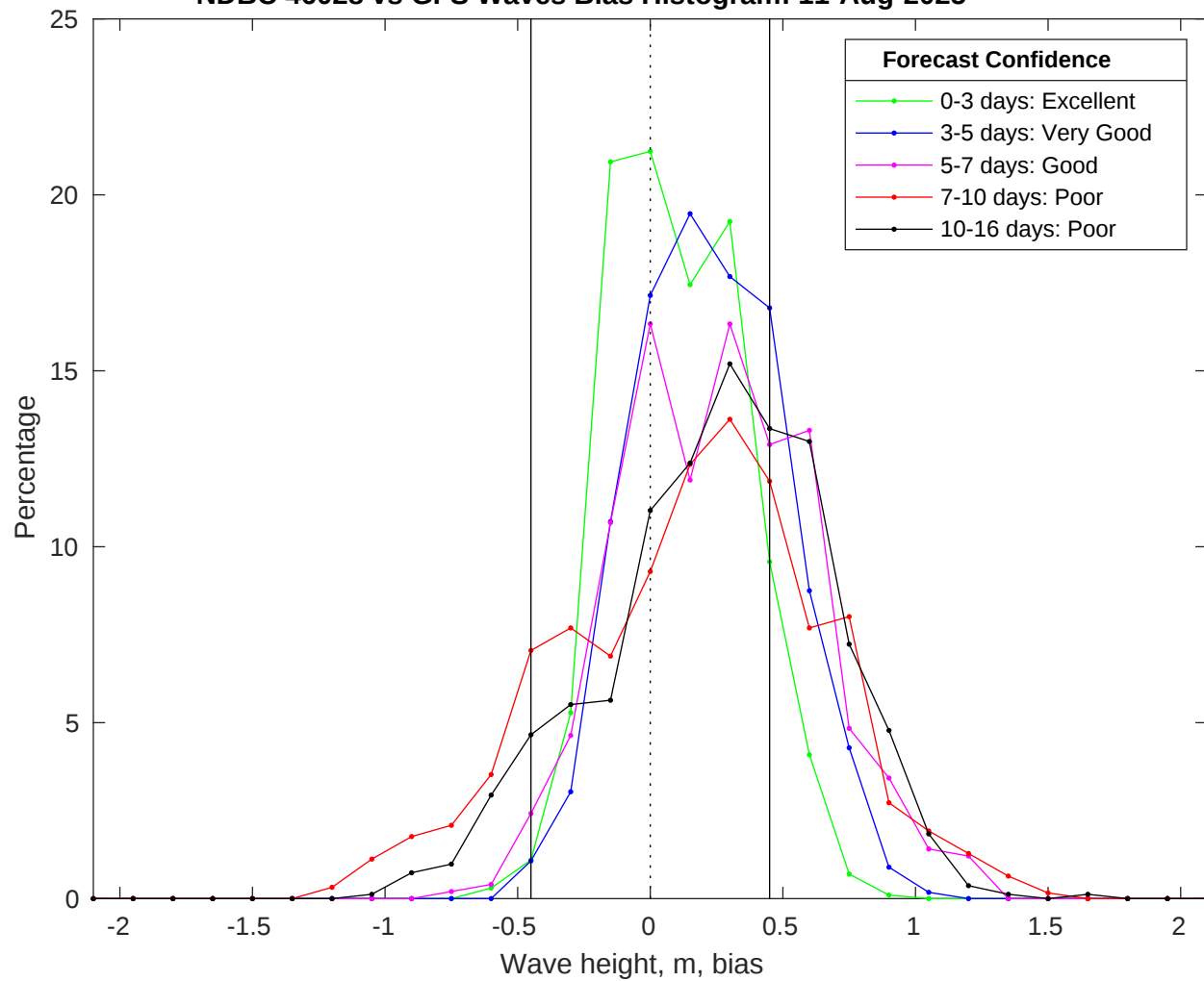
NDBC 46028 vs GFS Waves Bias Histogram: 11-Aug-2025
