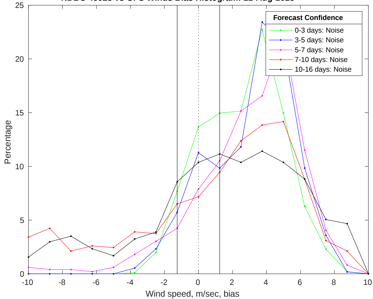
NDBC 46028 vs GFS Winds Bias Histogram: 11-Aug-2025
