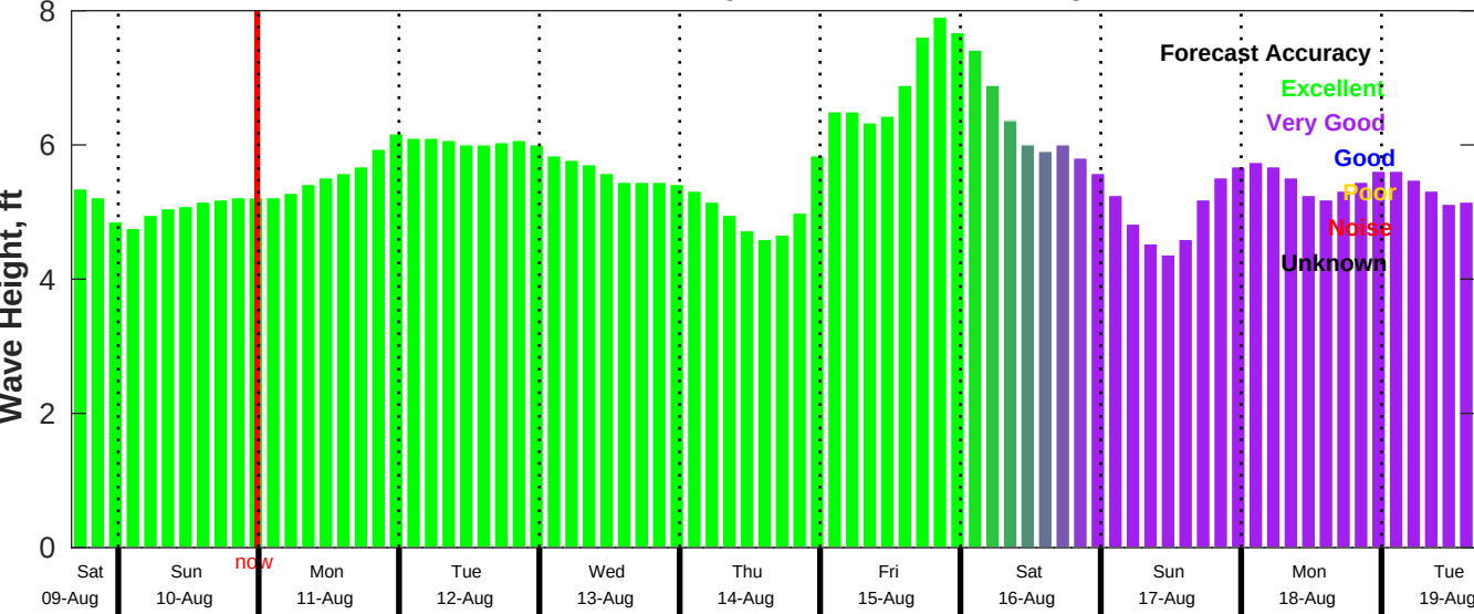
CMEMS Wave Forecast for NDBC 46028 from 09-Aug-2025 16:00:00 to 19-Aug-2025 16:00:00
